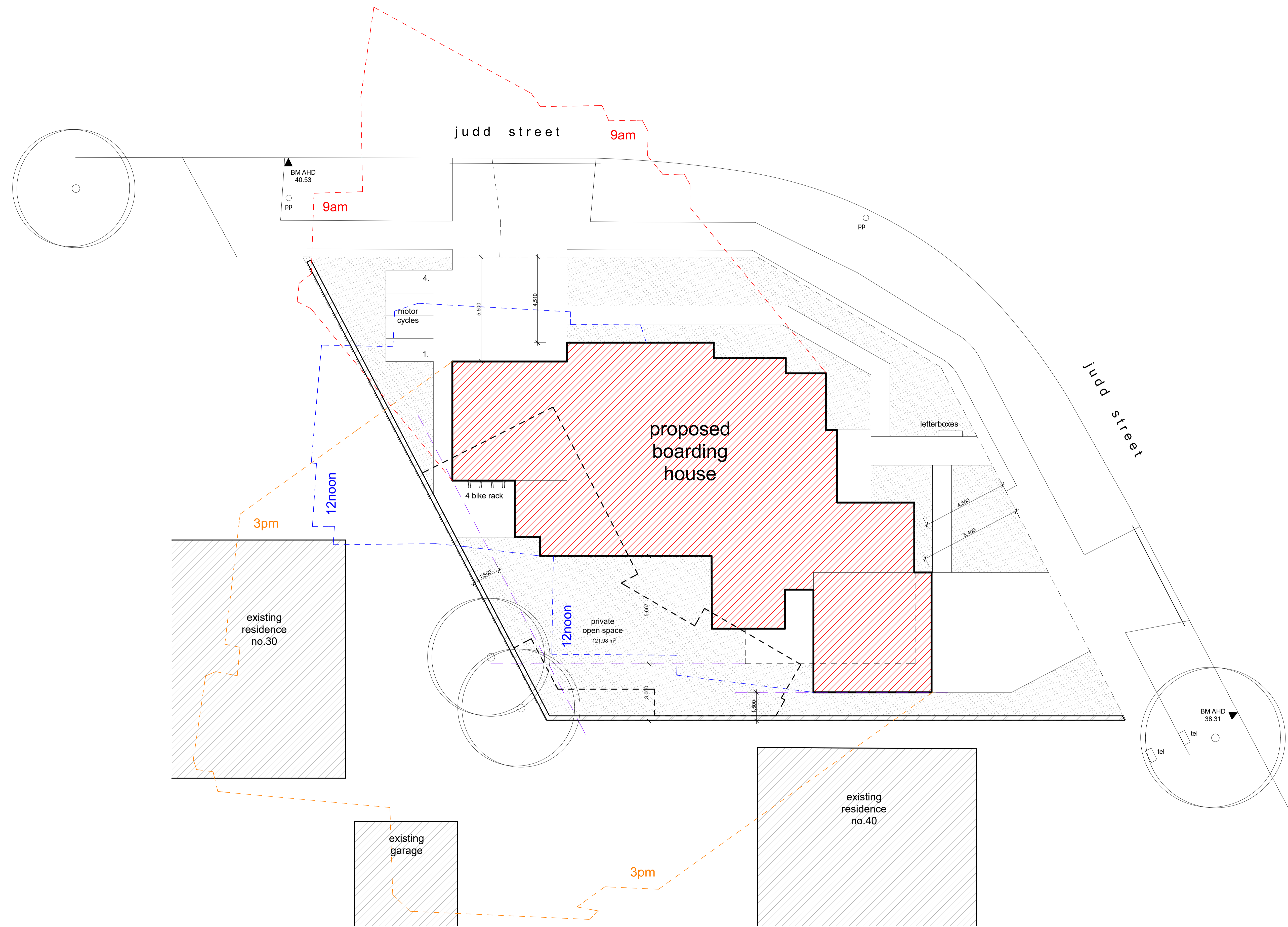
Shadow Diagram June 21 1:100
