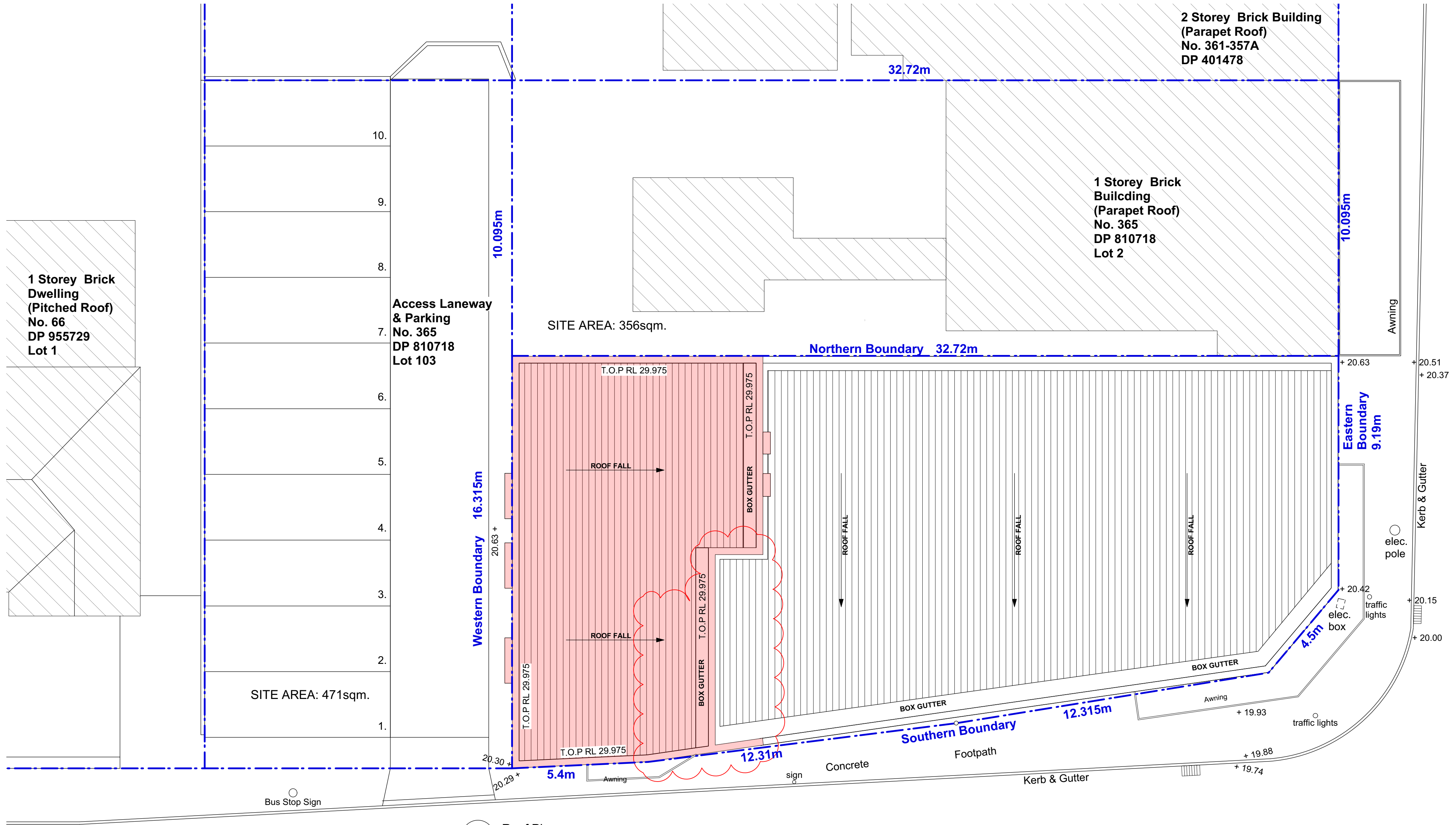
1 Roof Plan Scale 1:100
